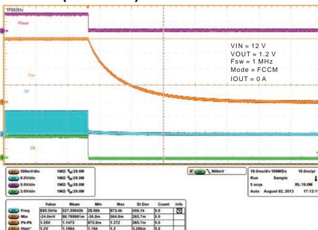
Figure 26. Shut-Down Operation
