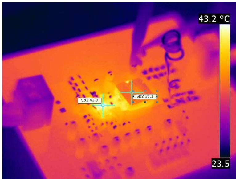
Figure 32. SP1: 43°C (TPS53513), SP2: 35.1°C (Inductor)
