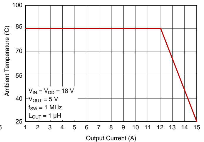
Figure 12. Safe Operating Area, V_{OUT} = 5 \text{ V}
