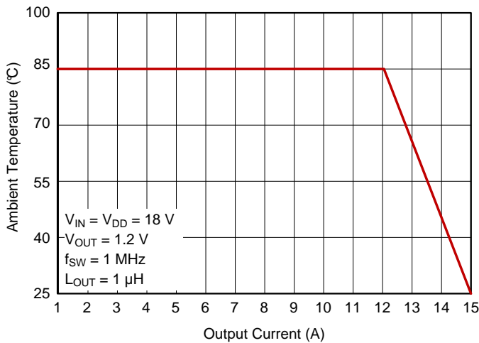
Figure 11. Safe Operating Area, V_{OUT} = 1.2 \text{ V}
