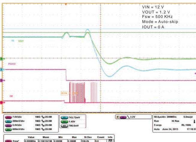
Figure 30. Overvoltage Protection
