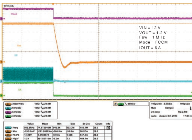
Figure 28. Shut-Down Operation
